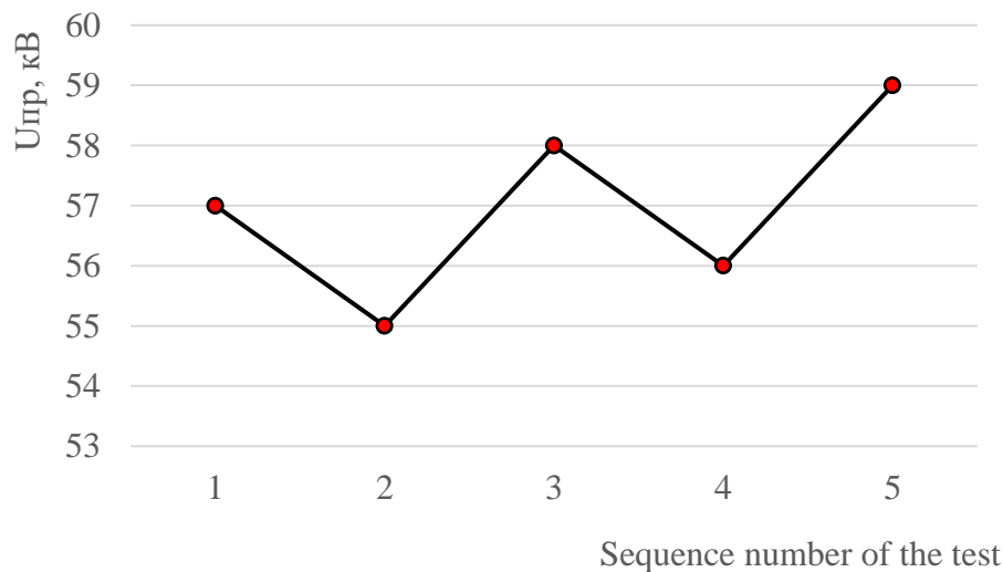
Fig.1. Graph of breakdown voltage of oil of power transformer TDN-63000/110
