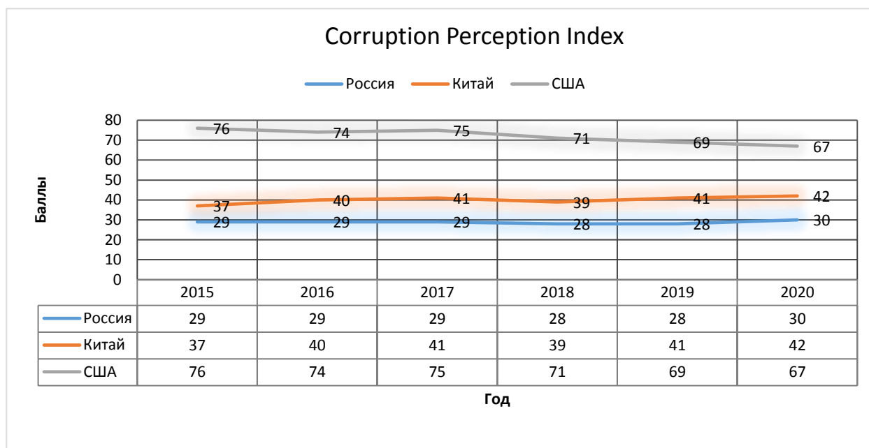
Figure 1. Corruption perception index for the period from 2015-2020
